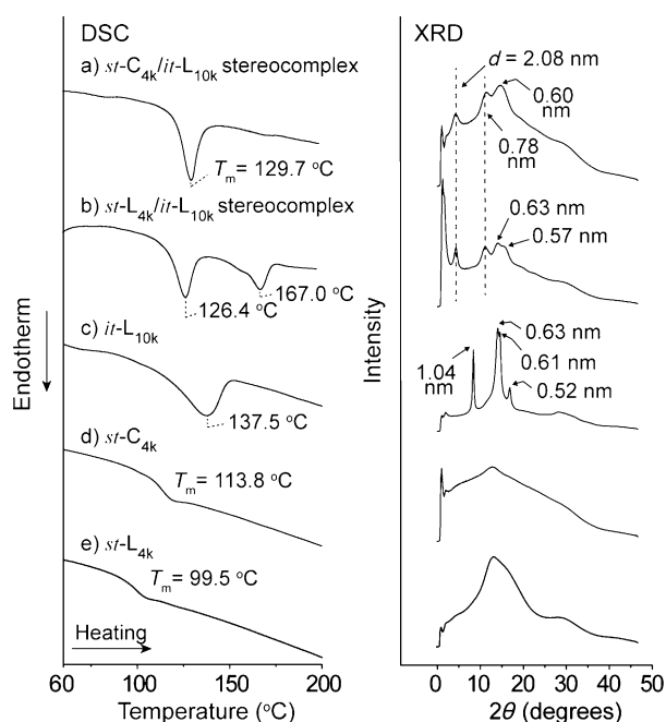
Figure 2. DSC thermograms and X-ray powder diffraction (XRD) patterns of a) the st -C 4k / it -L 10k stereocomplex, b) the linear st -L 4k / it -L 10k stereocomplex, c) the linear it -PMMA it -L 10k , d) the cyclic st -PMMA st -C 4k , and e) the linear st -PMMA st -L 4k .
