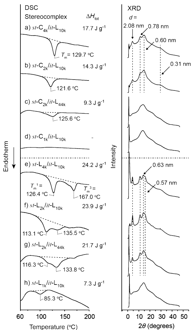
Figure 4. DSC and X-ray powder diffraction profiles of the c-st-/l-it -PMMA stereocomplexes a) st-C 4k / it-L 10k , b) st-C 2k / it-L 10k , c) st-C 2k / it-L 44k , and d) st-C 1k / it-L 10k , and the l-st-/l-it -PMMA-stereocomplex counterparts e) st-L 4k / it-L 10k , f) st-L 2k / it-L 10k , g) st-L 2k / it-L 44k , and h) st-L 1k / it-L 10k .
